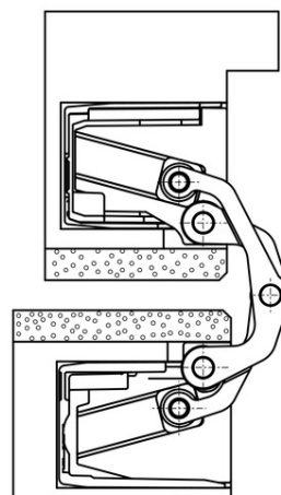
block frame 180°
